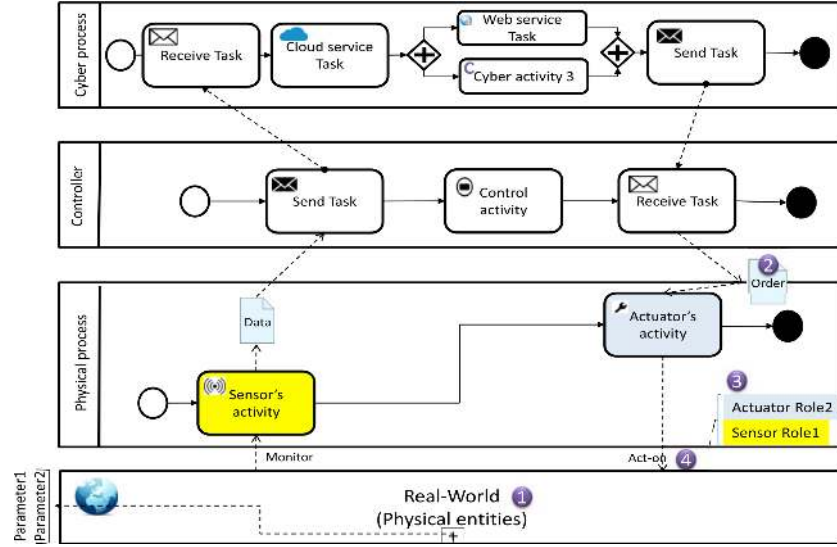
Figure 2.7: BPMN4CPS Example [22]
