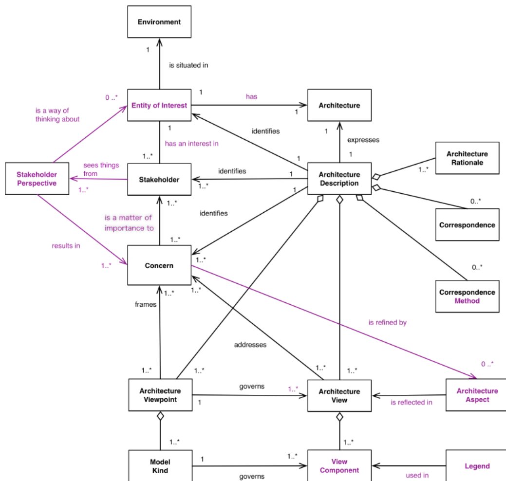
Figure 4.2: ISO/IEC/IEEE 42010 Conceptual Model 2022 Version [92]
