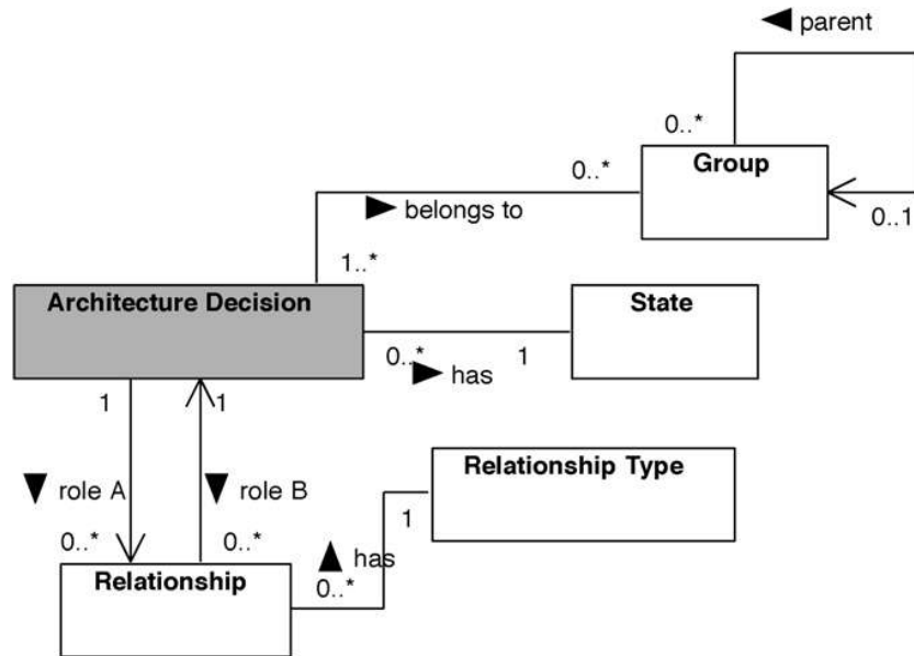
Figure 4.10: Meta model of Decision Relationship viewpoint [97]
