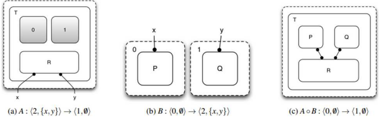
Figure 2.4: The composition A \circ B of two bigraphs A and B with their respective interfaces [15].
