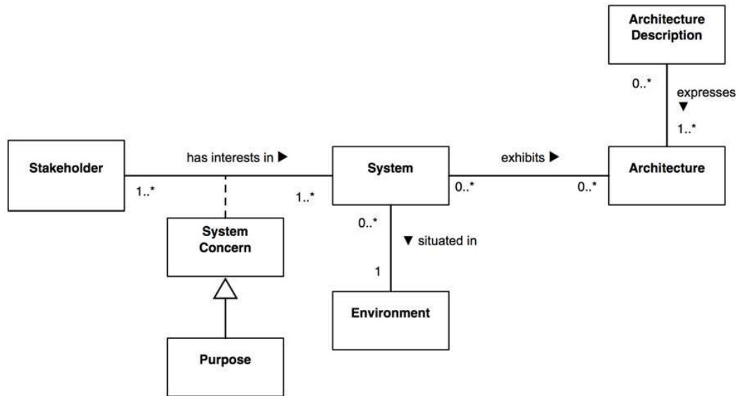
Figure 4.3: Context of architecture description [82]
