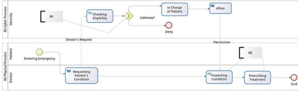
Figure 6.3: CA_{CPS} Behavior in terms of BPMN: Scenario 1
