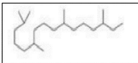
Figure 16 : Structure de phytane (Malecky, 2008)
