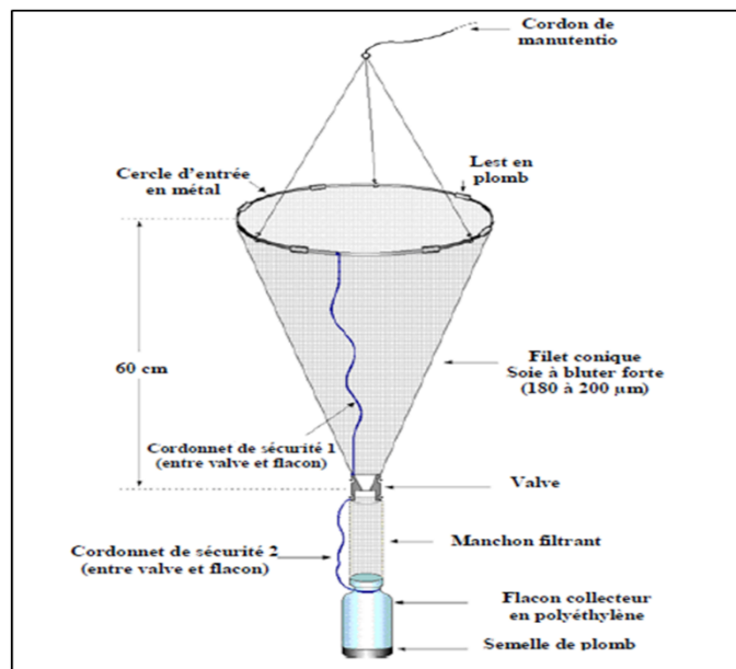
Fig. 2. Schematic of the phreatobiological net
