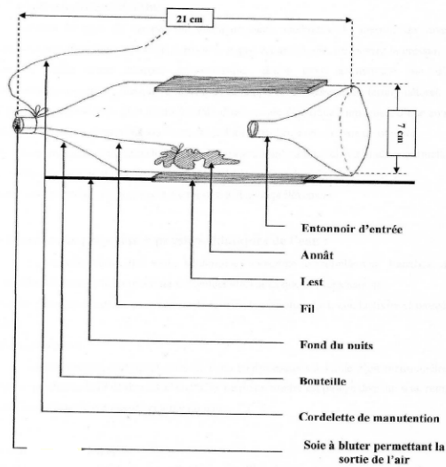
Fig. 3. Drawing of the baited trap
