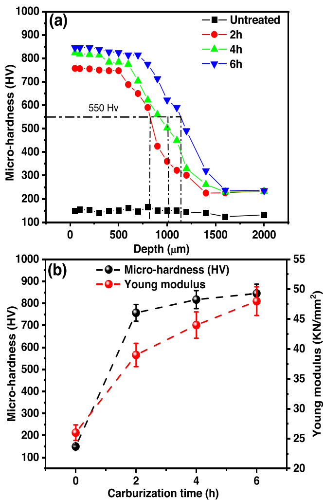
Figure 8. (a) The microhardness as a function of the penetration depth, (b) hardness and young modulus of XC 20 steel for different time of carburization.
