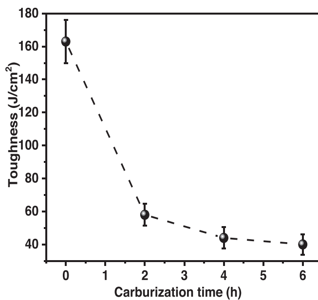
Figure 9. The effect of carburization time on the toughness of XC20 steel.
