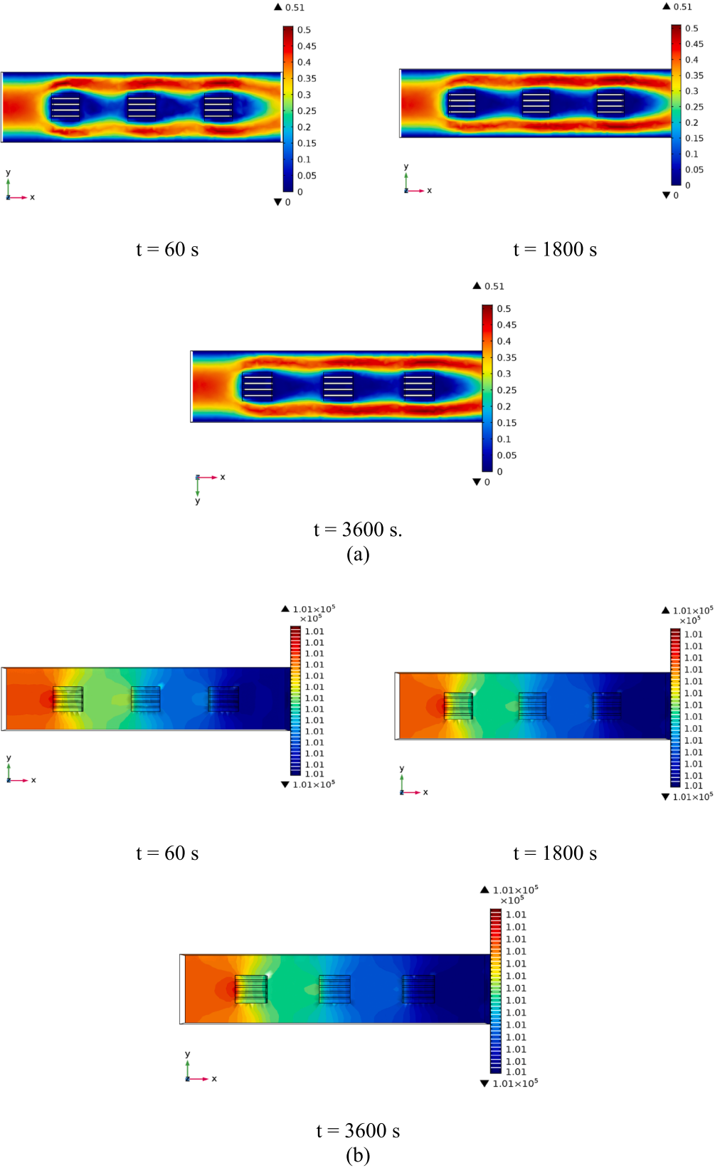
Fig. 9. Transient (a) air velocity and (b) pressure inside the channel.
