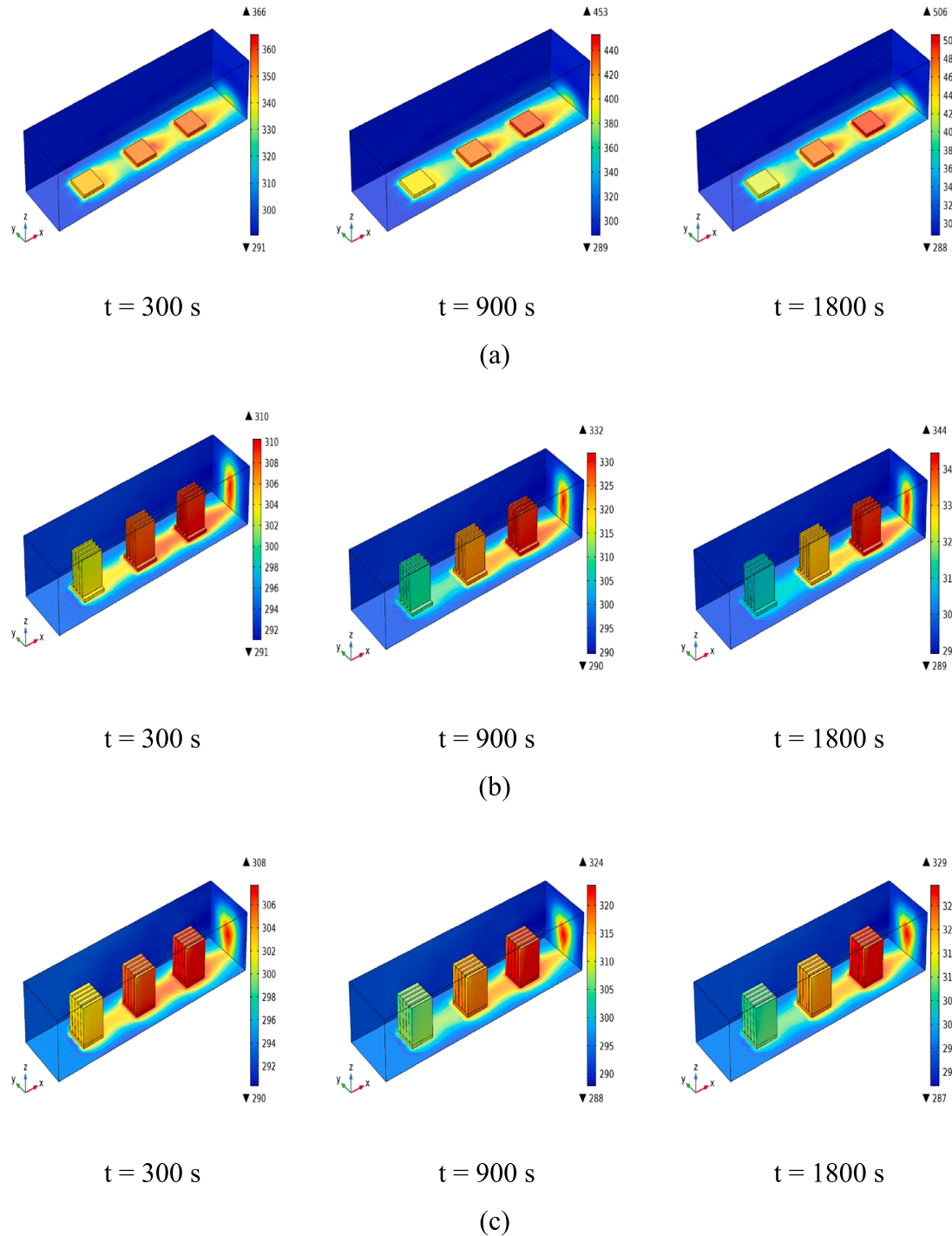
Fig. 5. Comparison of temperature distributions for (a) a clear channel and a channel with (b) FAHS and (c) FAFHSs; q_w = 4 W and inlet air velocity U_{in} = 0.21 m/s.
