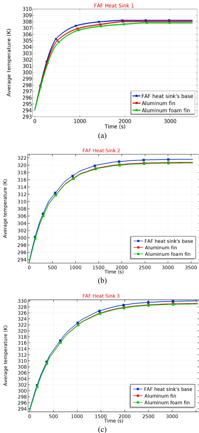
Fig. 8. Transient temperatures of the FAFHSs and thermal sources.
