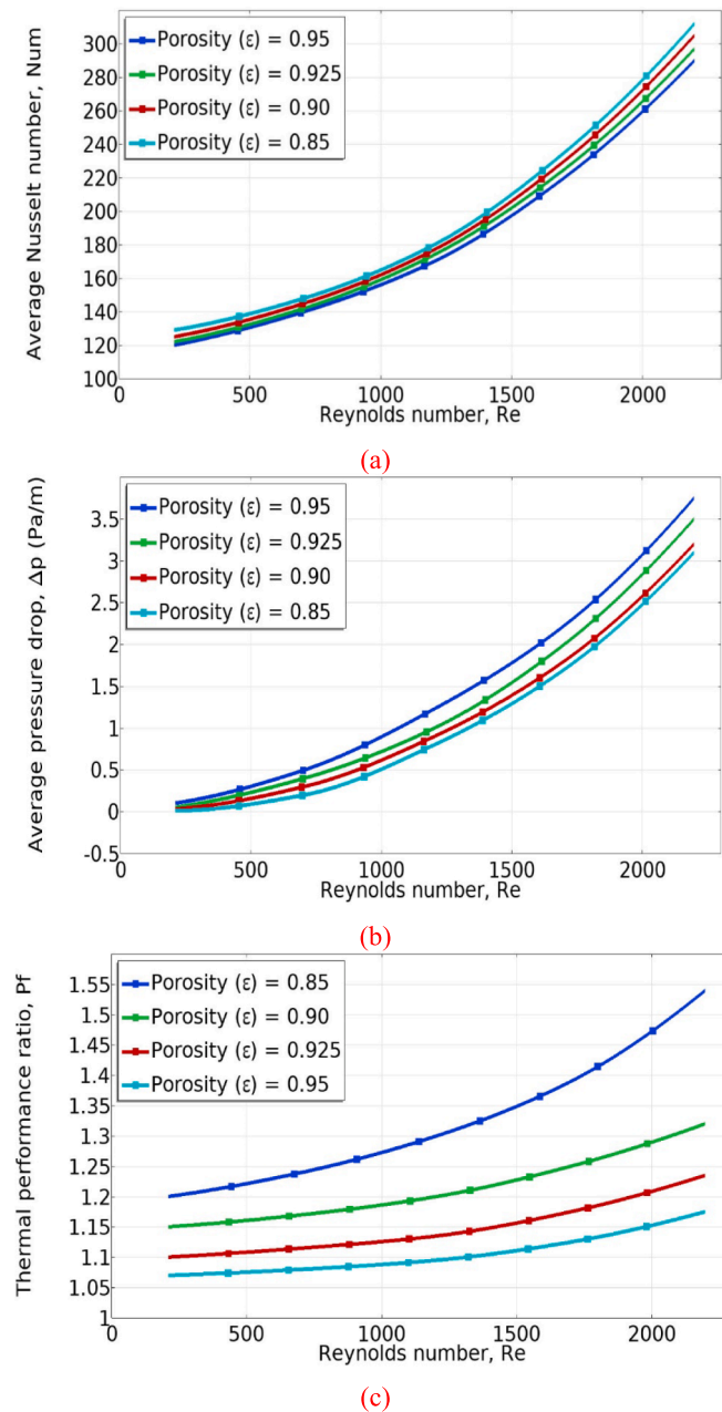
Fig. 10. Porosity effect on the thermal fluid characteristics for the first air-cooled FAFHS with heat input of 4 W: (a) average Nusselt number, (b) average pressure drop, and (c) thermal performance ratio.
