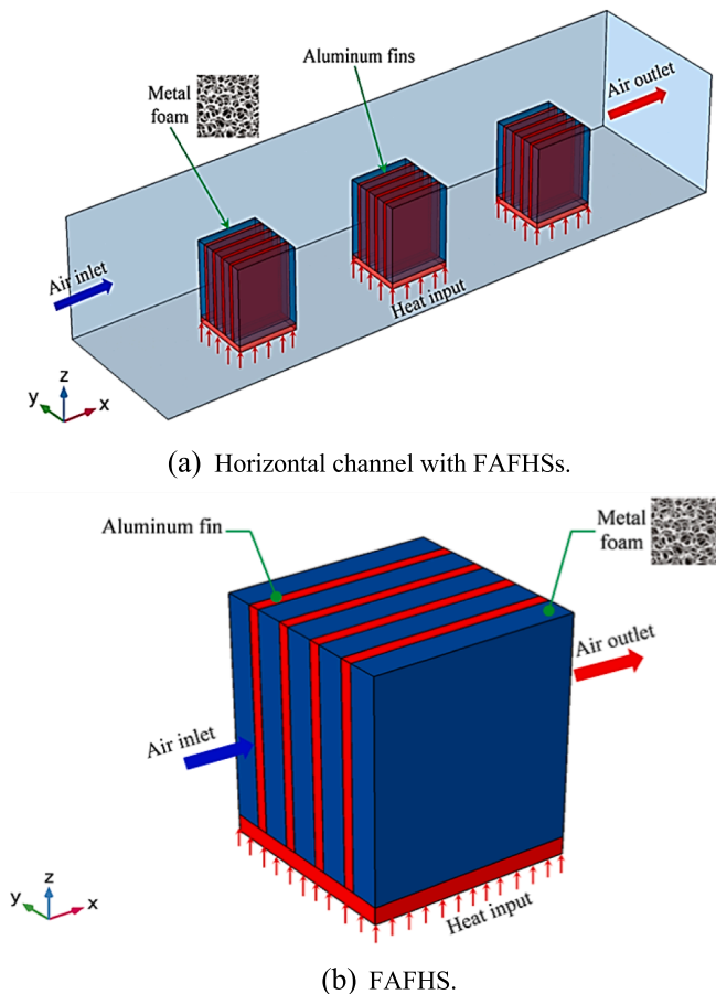
Fig. 1. Principal diagram of (a) horizontal channel with FAFHSs, and (b) FAFHS.
