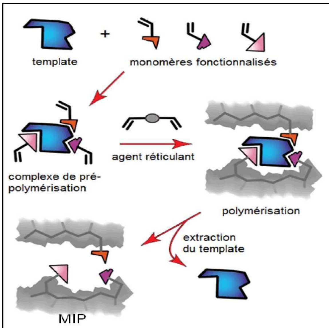
Figure 0.23: Principe de polymérisation
