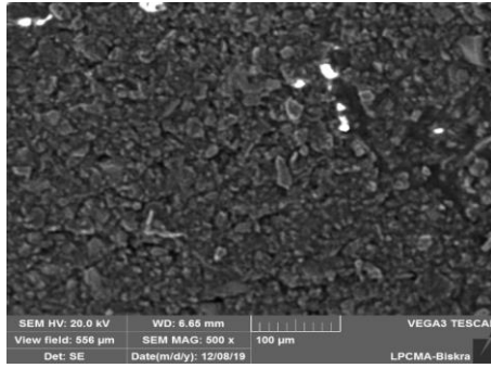
Figure 7. SEM micrograph transverse view of Diss fiber in its raw state
