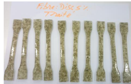
Figure 11. Tensile specimens reinforced with 05% treated Diss fiber
