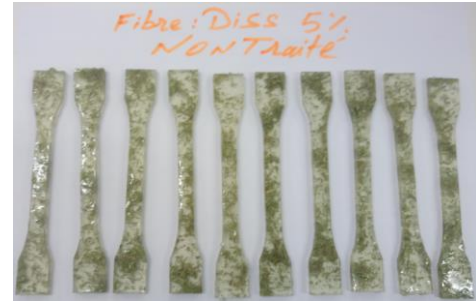
Figure 10. Tensile specimens reinforced with 05% untreated Diss fiber
