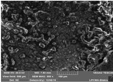
Figure 8. SEM micrograph transverse view of Diss fiber after treatment with NaOH
