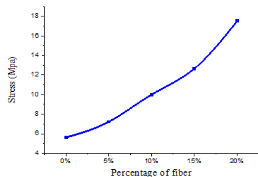
Figure 13. Variation of the stress at break as a function of the fiber rate of Diss
