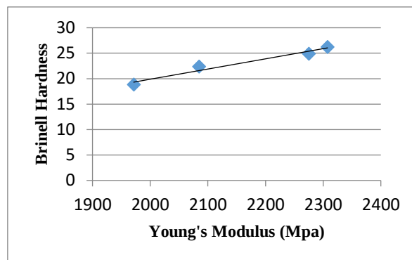
Figure 18. Evolution of Brinell hardness and Young's Modulus
