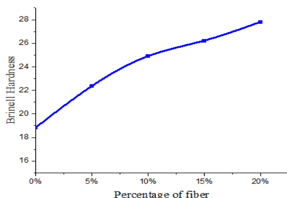
Figure 16. Change in Brinell hardness with volume fraction of Diss fibers
