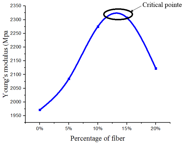
Figure 14. Variation of the Young's modulus E as a function of the fiber rate of Diss (from 0% to 20%)
