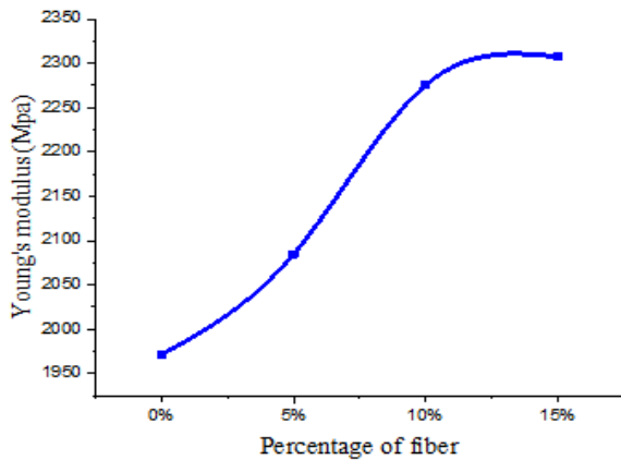
Figure 15. Variation of the Young's modulus E as a function of the fiber rate of Diss (0% -15%)
