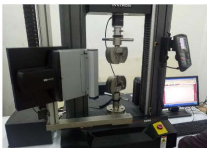
Figure 3. Instron 6959 brand traction machine
