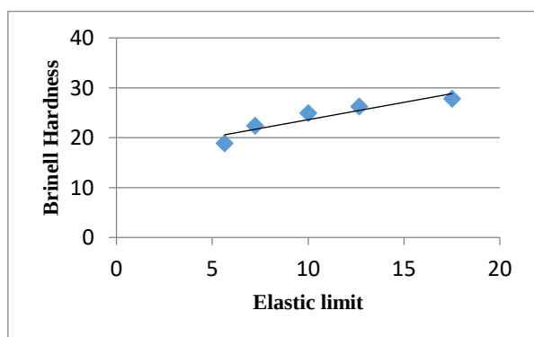
Figure 17. Evolution of Brinell hardness and elastic limit
