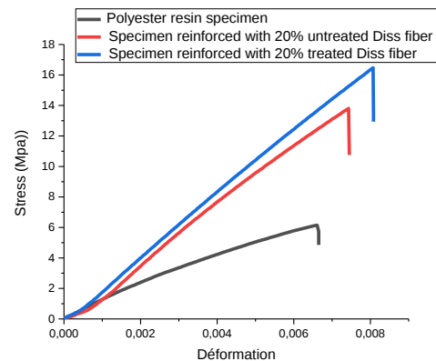
Figure 12. Stress-strain curve of the resin and at 20% of treated and untreated Diss fibers
